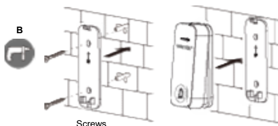
Screws
